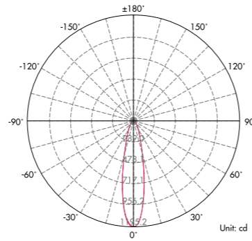
Lux distance Curve (3000K, 24°)
