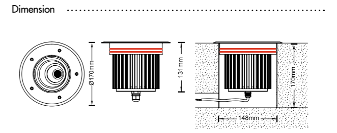
Dimension .....
