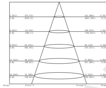
Illumination Picture (10°)
