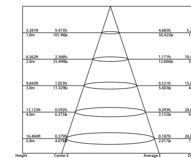
Illumination Picture (1x120°) .....
