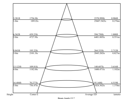
Illumination Picture (15x15°) .....
