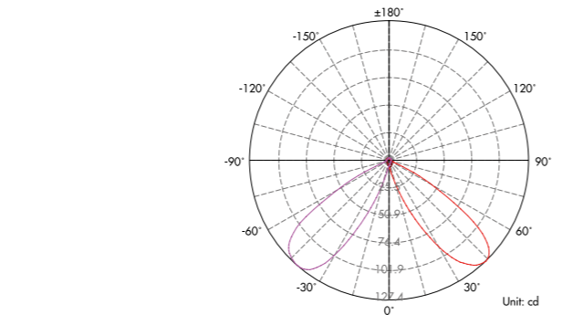
Light Distribution Curve (3000K, 30°) .....
