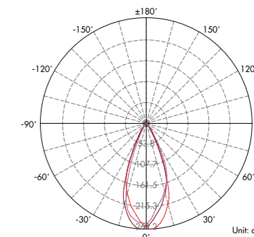
Lux distance Curve (3000K, 8°)
