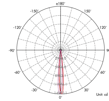
Lux distance Curve (3000K,20°) .....
