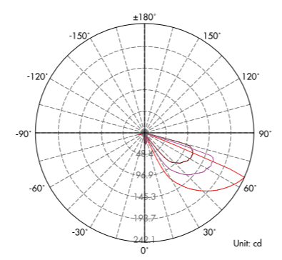
Lux distance Curve (3000K, 7W, 50°x40°)
