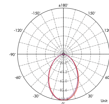
Lux distance Curve (3000K, 1x120°) .....
