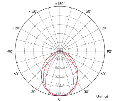
Lux distance Curve (3000K, 36°)
