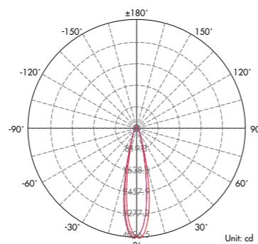
Lux distance Curve (15°) .....
