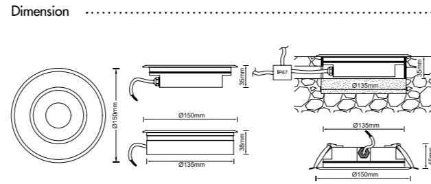
Dimension .....
