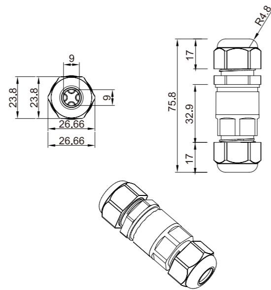
Dimension .....
