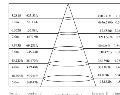
Illumination Picture (10°) .....
