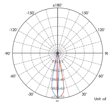
Lux distance Curve (3000K,22°) .....
