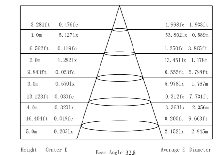
Illumination Picture (30°) .....
