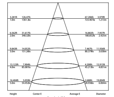
Illumination Picture (15x70°) .....
