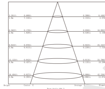
Illumination Picture (100°) .....
