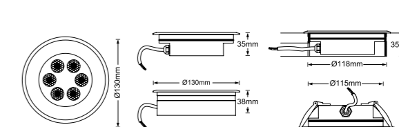
Dimension .....
