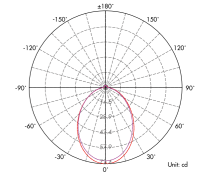
Lux distance Curve (RGB all LEDs on, 1x120°) .....
