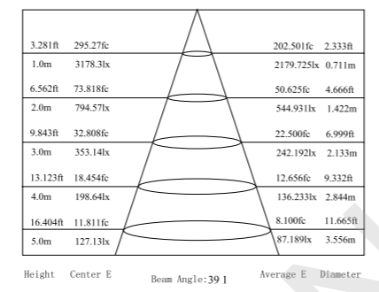
Illumination Picture (40°) .....
