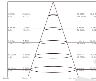
Illumination Picture (110°) .....
