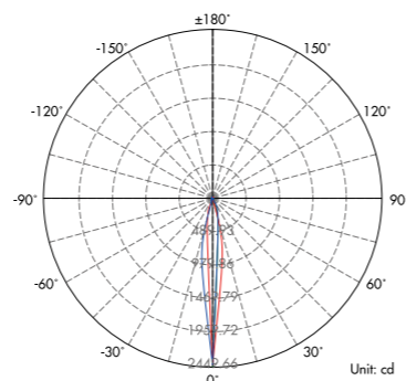
Lux distance Curve (3000K,60°) .....
