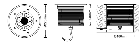
Dimension .....
