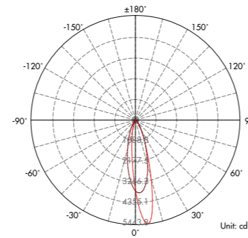
Lux distance Curve (3000K, 15°40°) .....
