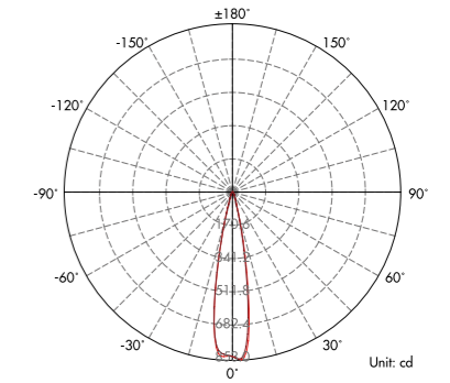
Lux distance Curve (3000K, 25°) .....
