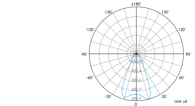
Light Distribution Curve (3000K, 60°)
