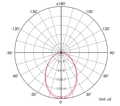
Lux distance Curve (3000K, 1x120°) .....
