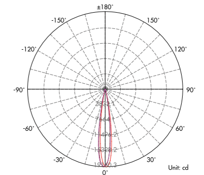
Lux distance Curve (3000K,15°) .....
