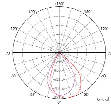
Lux distance Curve (3000K, 15x70°) .....
