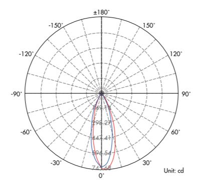
Lux distance Curve (3000K, 36° COB reflector) .....
