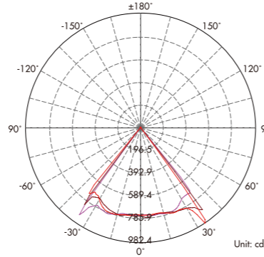
Lux distance Curve (3000K, 70°) .....
