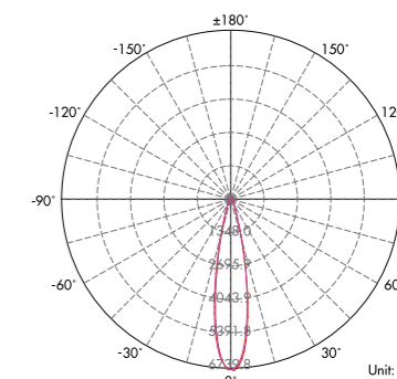
Lux distance Curve (17°) .....
