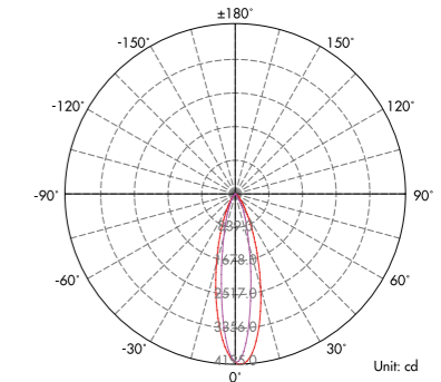
Lux distance Curve (3000K, 15°40°) .....
