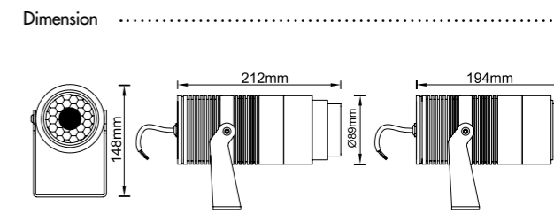
Dimension .....
