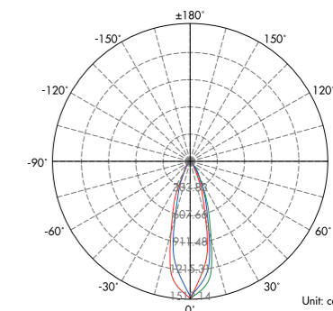
Lux distance Curve (3000K,40°) .....
