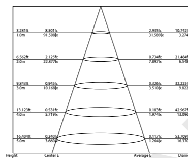
Illumination Picture (120°) .....
