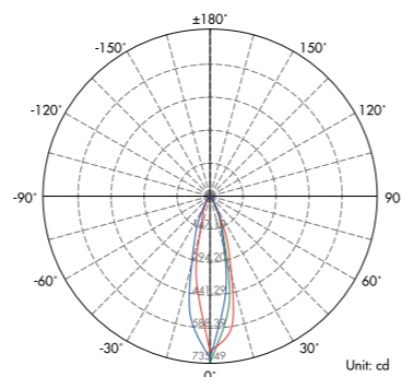
Lux distance Curve (3000K, 1x25°) .....
