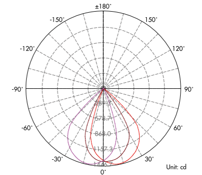
Lux distance Curve (3000K, 15x70°) .....
