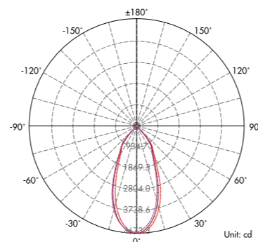
Lux distance Curve (3000K, 1x38°) .....
