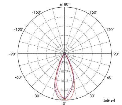
Lux distance Curve (3000K, 43°)
