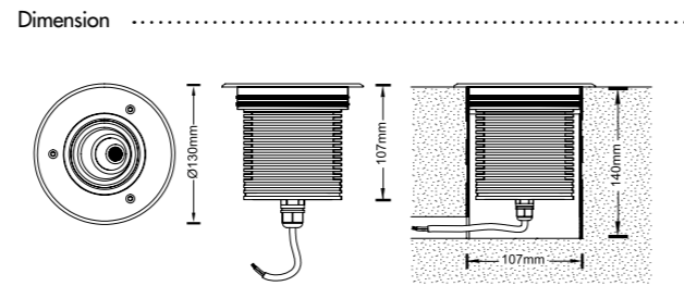
Dimension .....
