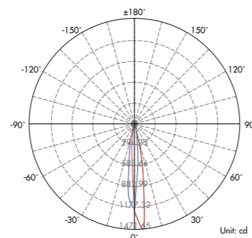
Lux distance Curve (3000K, 20°)
