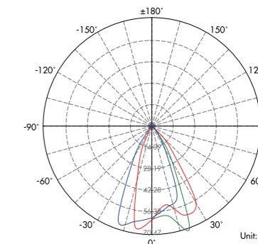
Lux distance Curve (3000K, 1x30°) .....
