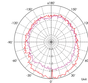
Lux distance Curve (3000K, 120°)
