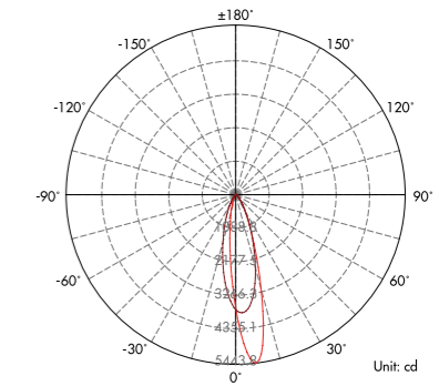
Lux distance Curve (3000K, 15°40°) .....
