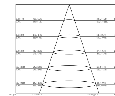
Illumination Picture (10°) .....
