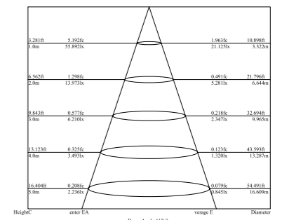
Illumination Picture (120°)
