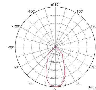
Lux distance Curve (3000K, 1x24°) .....
