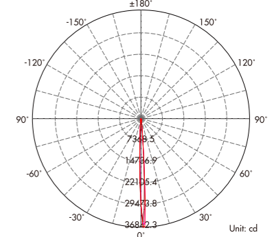
Lux distance Curve (3000K, 3°)
