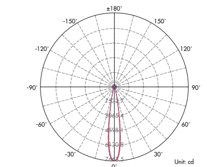
Lux distance Curve (3000K, 10° COB lens) .....
