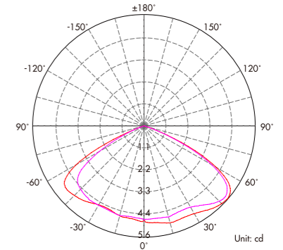
Lux distance Curve (3000K, 130°) .....
