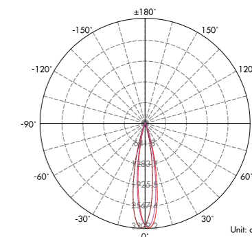
Lux distance Curve (3000K,25°) .....
