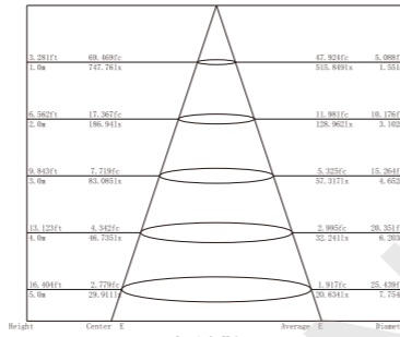
Illumination Picture (70°) .....
