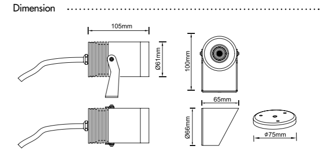
Dimension
