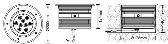
Dimension .....
