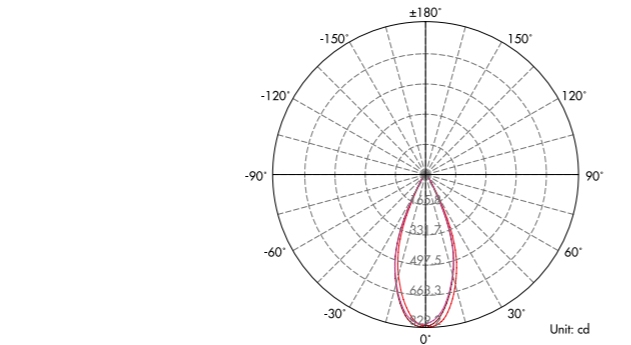
Light Distribution Curve (3000K, 40°)
