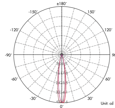
Lux distance Curve (3000K, 15°)
