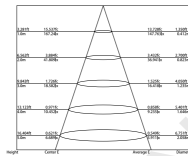
Illumination Picture (1x24°) .....
