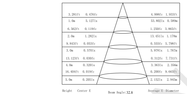
Lux distance Curve (3000K, 30°) .....
