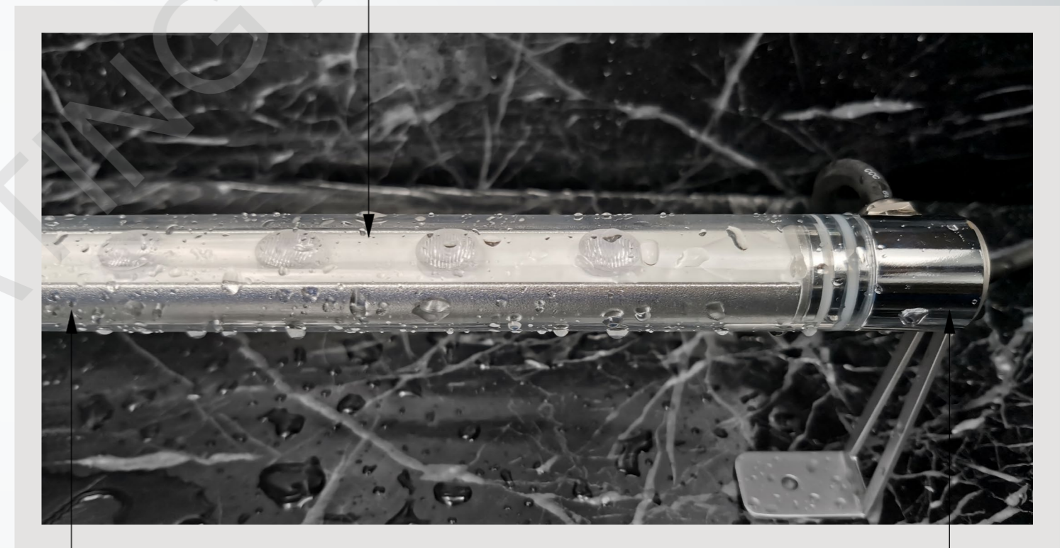
Inside PC tube with Aluminium housing Glue+structrue waterproof IP68
