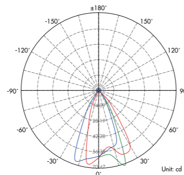
Lux distance Curve (3000K, 25°) .....
