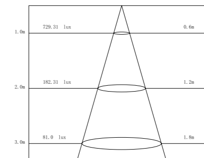
Illumination Picture (36°) .....
