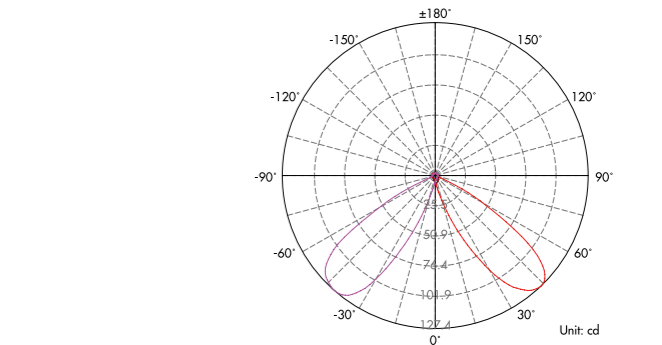
Light Distribution Curve (3000K, 30°) .....
