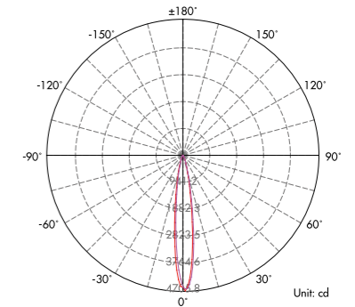
Lux distance Curve (3000K, 10°) .....
