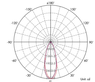
Lux distance Curve (3000K, 1x38°)
