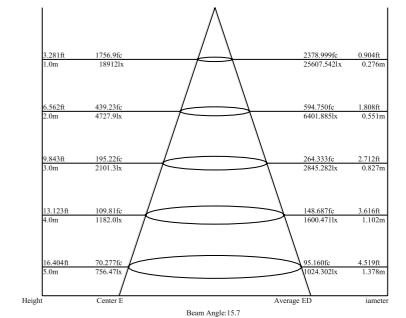
Illumination Picture (15°) .....
