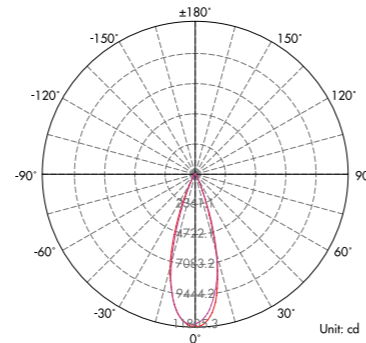
Lux distance Curve (3000K, 28°) .....
