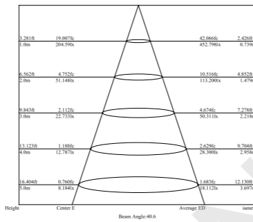
Illumination Picture (Assymetrical 30° tilt +120° pan beam)
