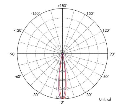
Lux distance Curve (3000K, 15x15°) .....
