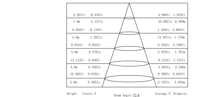
Lux distance Curve (3000K, 30°) .....
