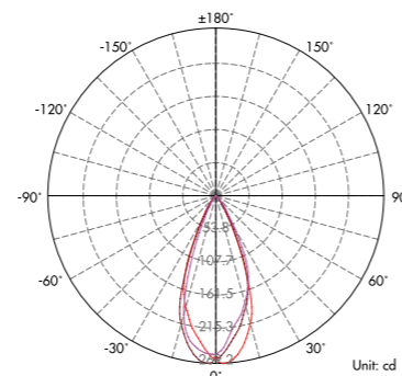
Lux distance Curve (3000K, 58°)
