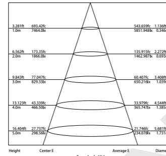
Illumination Picture (15x40°) .....
