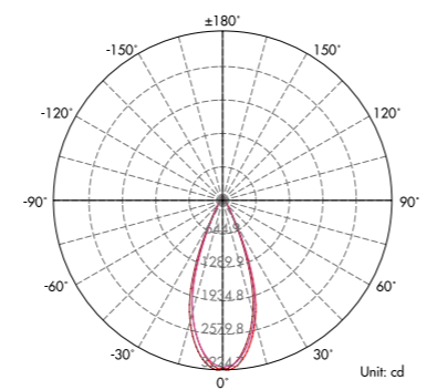
Lux distance Curve (3000K, 40°) .....
