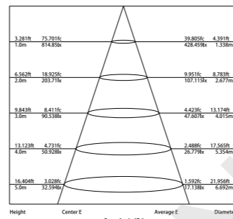
Illumination Picture (15x70°) .....
