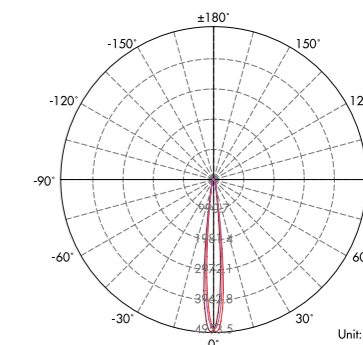
Lux distance Curve (3000K, 10°) .....
