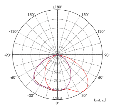
Lux distance Curve (3000K, 7W, 120°)
