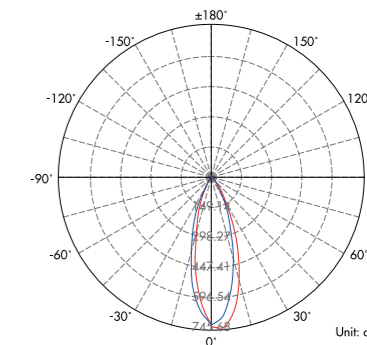
Lux distance Curve (3000K,36°) .....
