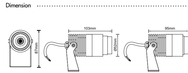
Dimension
