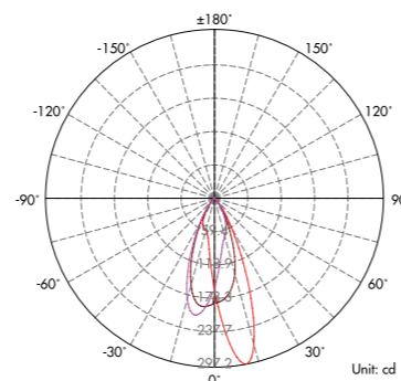
Lux distance Curve (3000K, 1x24°) .....
