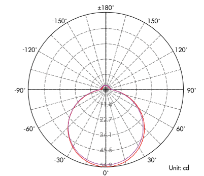
Lux distance Curve (3000K, 120°)
