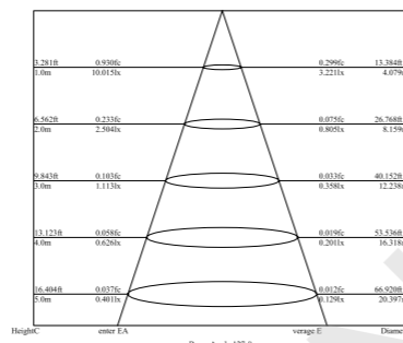
Illumination Picture (120°)
