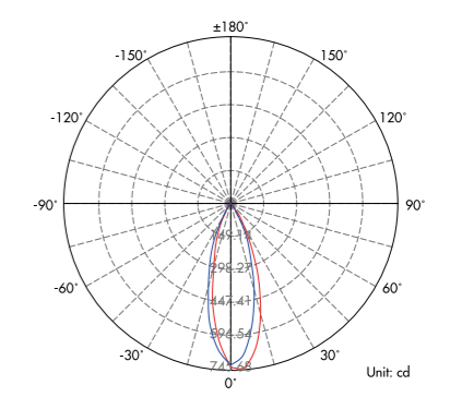
Lux distance Curve (3000K, 36° COB reflector) .....
