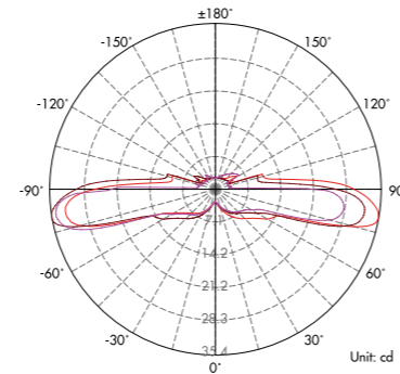
Lux distance Curve (3000K, 360°) .....
