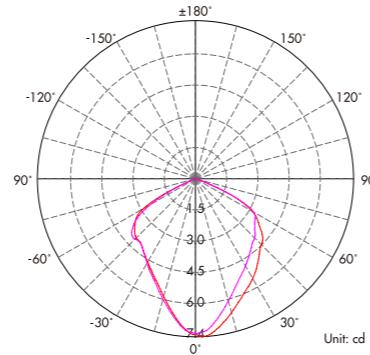
Lux distance Curve (3000K, 100°) .....
