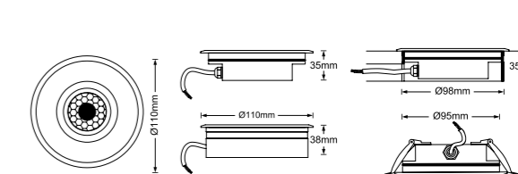
Dimension .....
