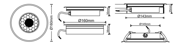
Light Distribution Curve (3000K,20°) .....
